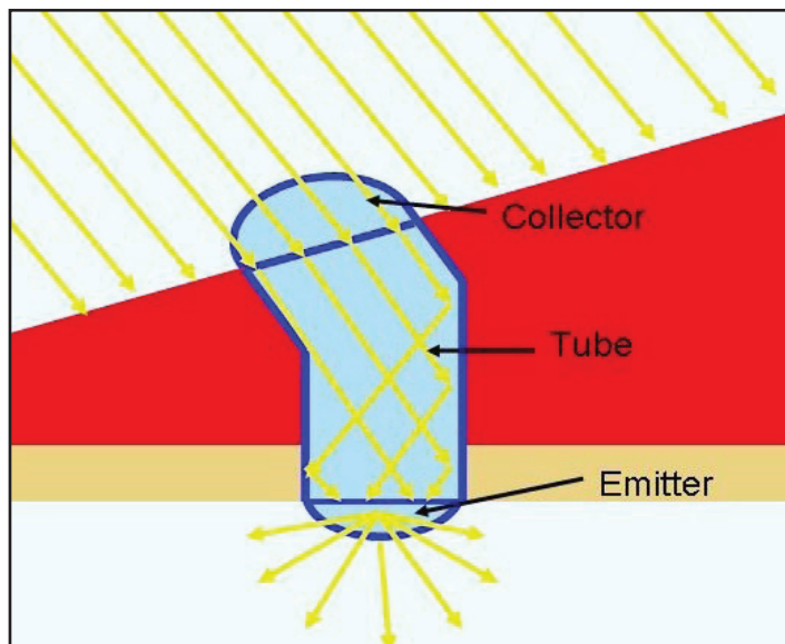
Figure 1: Light Pipe Schematic
