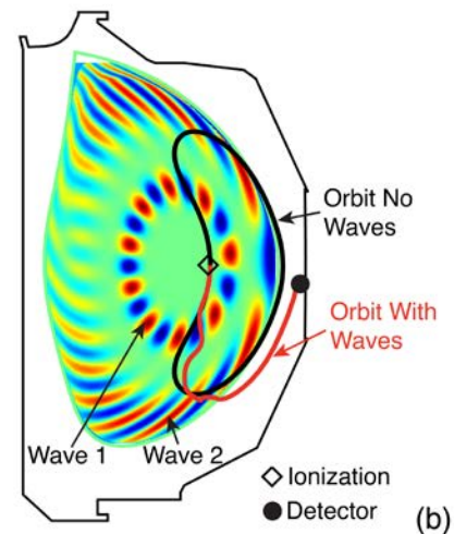
Figure 1: (a) Cartoon showing influence of one wave on the losses caused by another. (b) Similar situation for losses induced by two different waves in a fusion device and how those particles can hit a detector designed to measure them.
